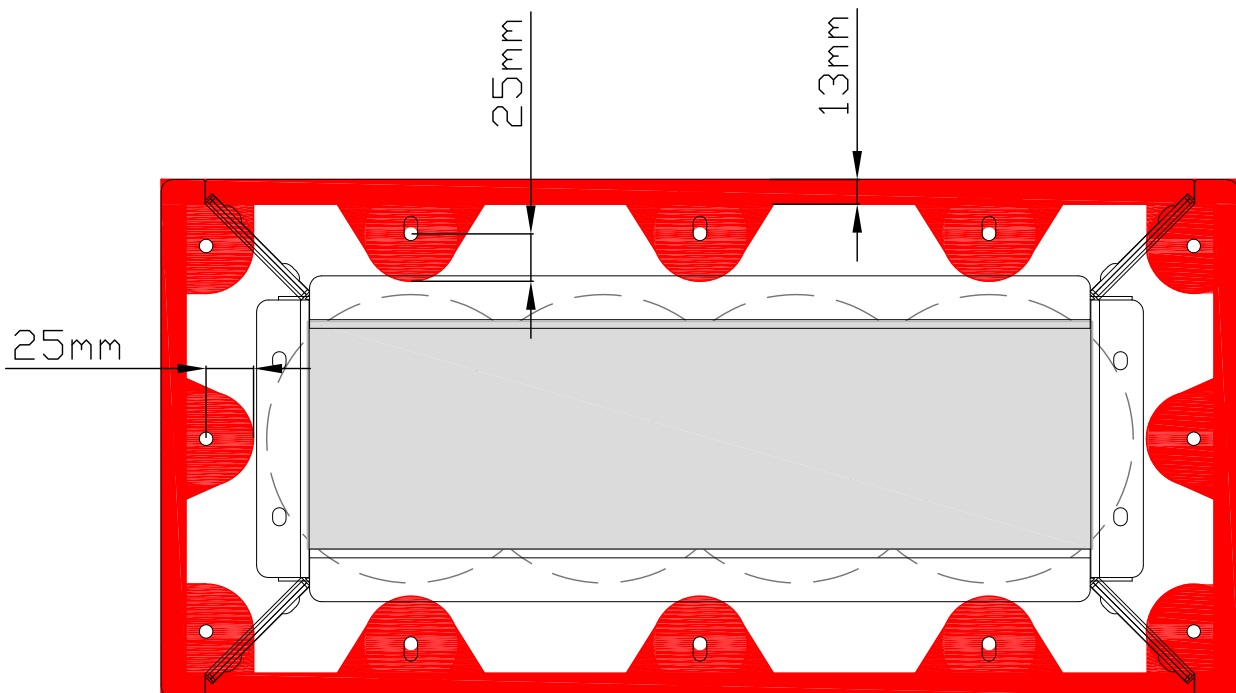
Minimum overlapping of the grid over concrete
