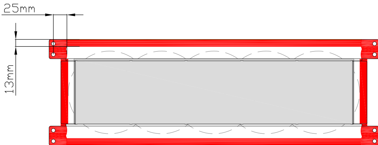
Minimum overlapping of the plate over concrete
